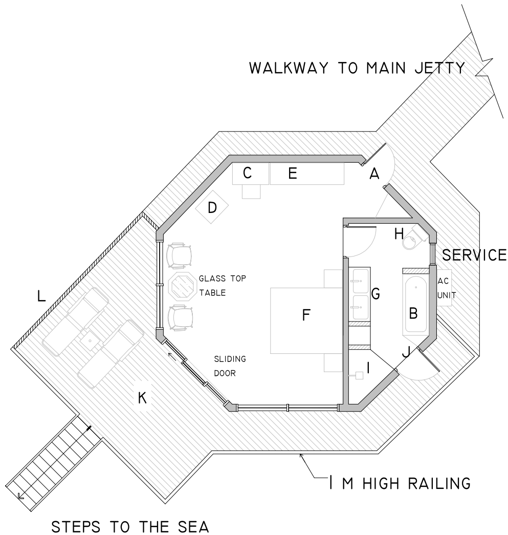
SUPERIOR WATER BUNGALOWS FLOOR PLAN
